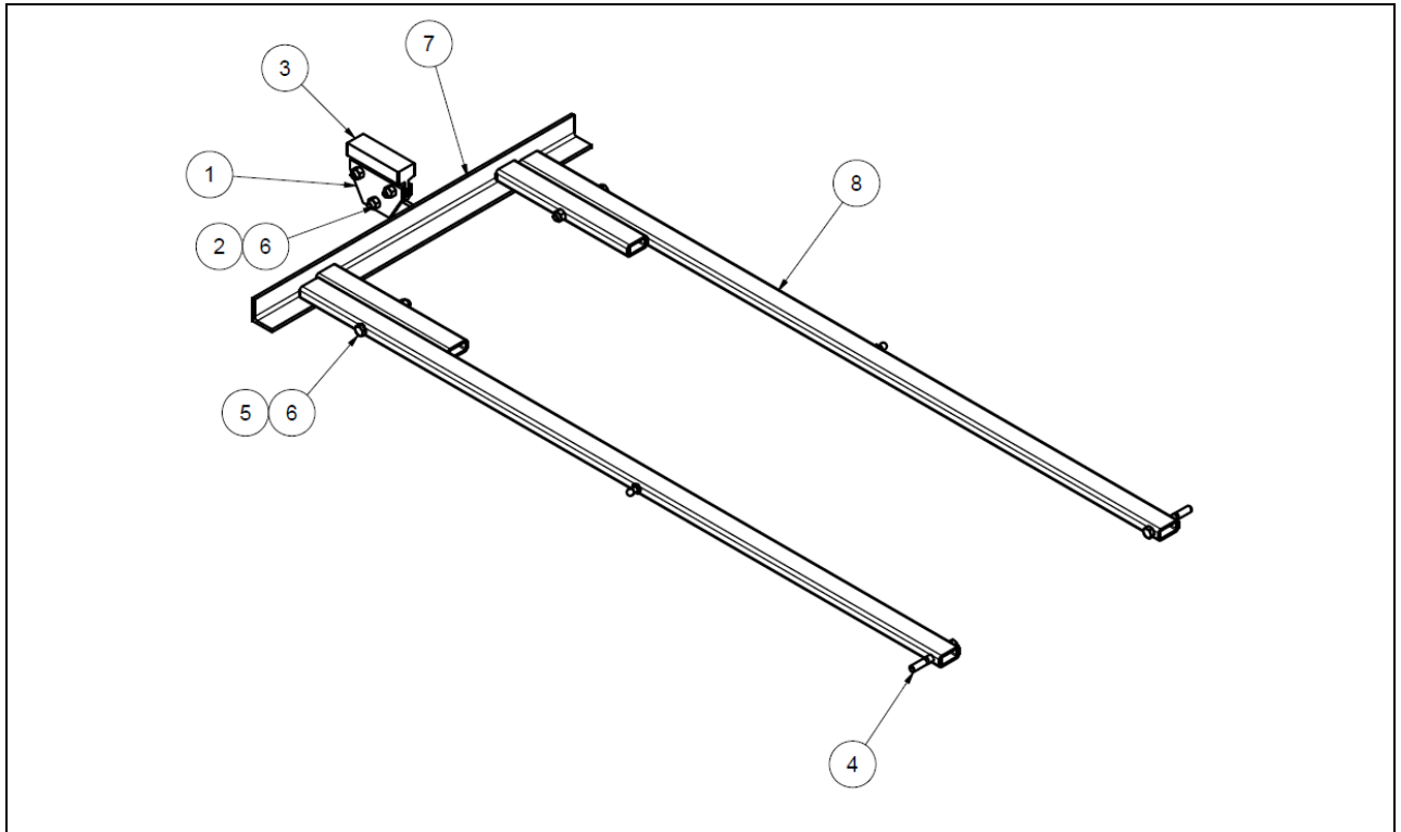
Trolley Pivot Assembly, LP Model "C"
