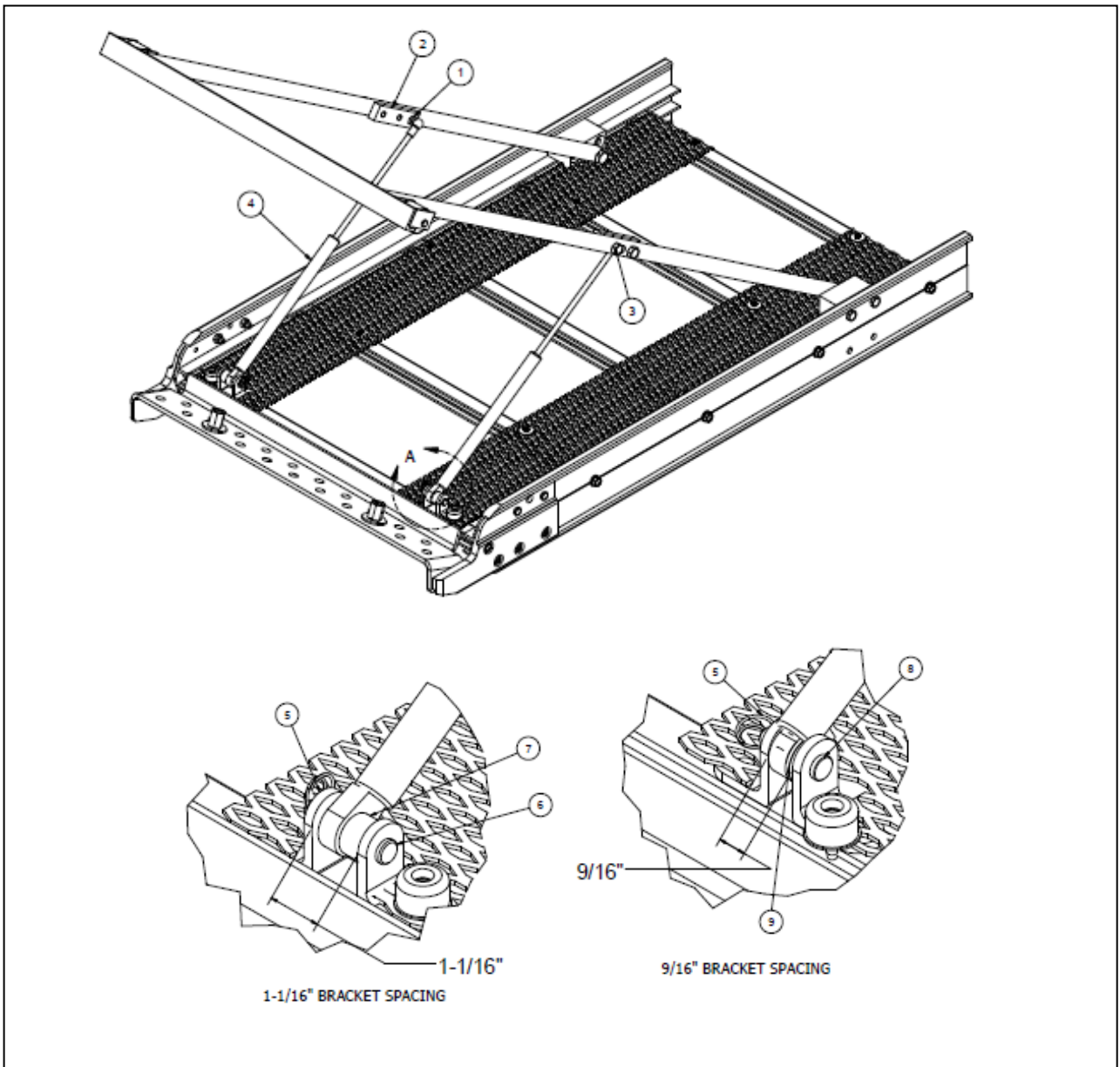
Gas Spring Retrofit Kit, Part No. R01147-3
